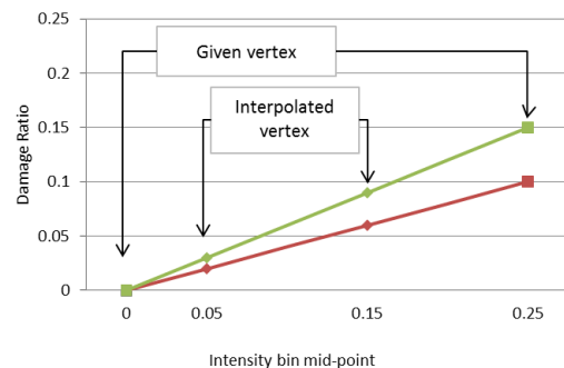
Figure 17 - Intensity Interpolation
