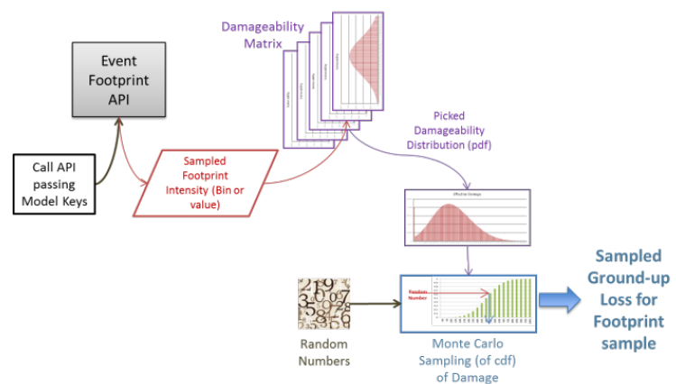
Figure 20 - Ensemble Method
