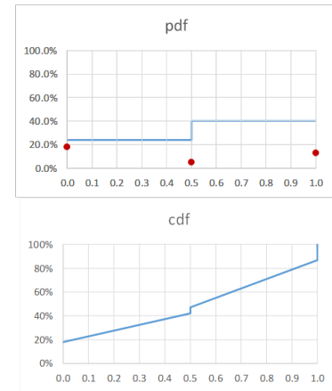
Figure 26 - Linear cdf
