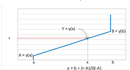
Figure 27 - Linear Interpolation
