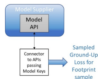
Figure 10 - "Full API"
