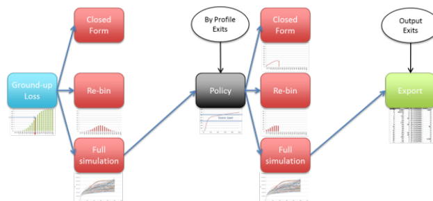
Figure 7 - Oasis General Calculation Architecture
